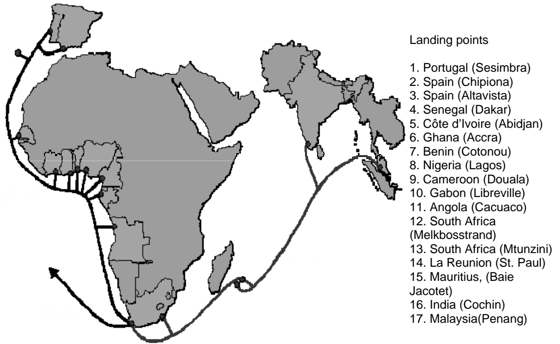
Figure 3.3 SAT3 fiber cable routing with landing points. Source: Fibre for Africa, 2007c
