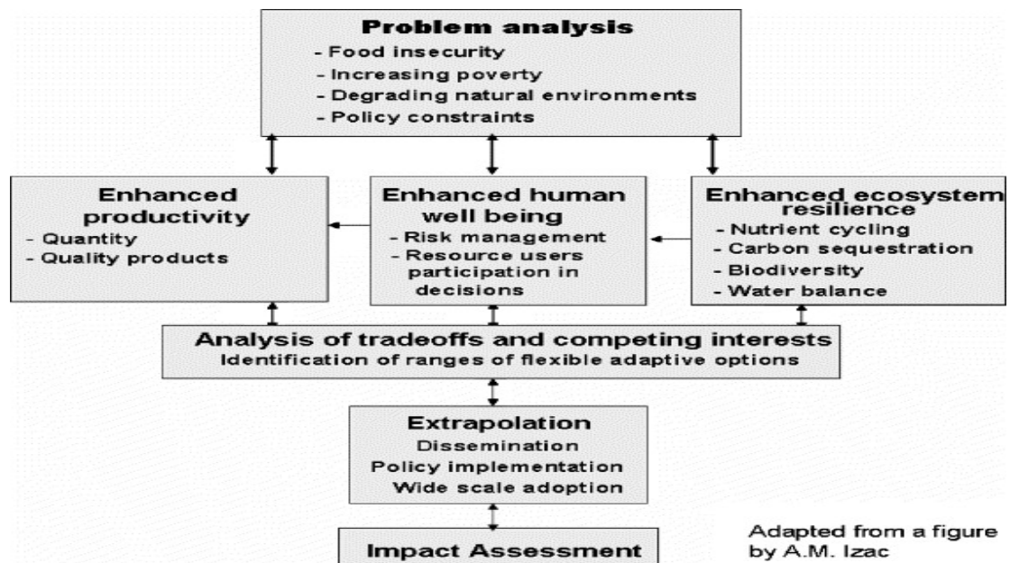
Figure 3.2 INRM approach
